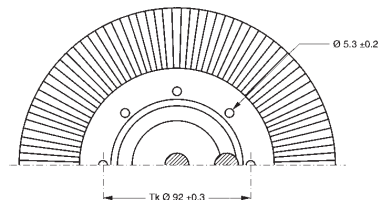
Top view (dimensions in mm)
