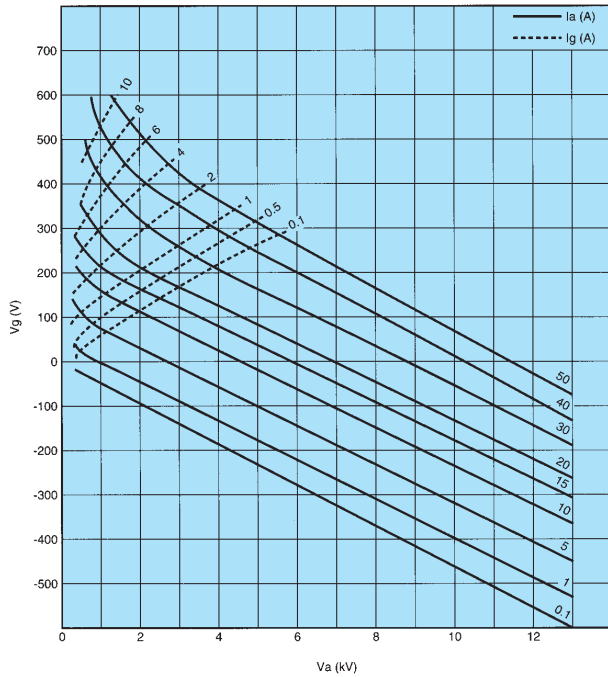
Constant current characteristics
